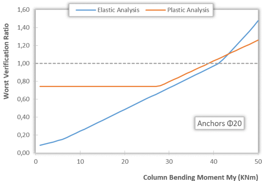
Figure 2. Plots of the calculated worst verification ratio (maximum) versus the applied column bending moment under elastic and plastic analysis.
