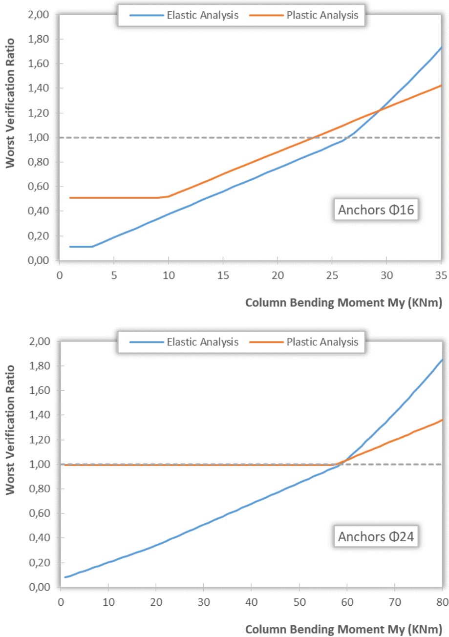
Figure 3. Investigation of the relative strength of anchors to the foundation concrete for the worst verification ratio plots.
